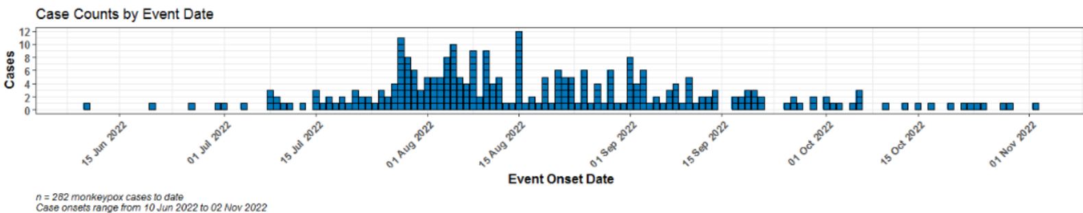
Figure 1: Monkeypox Virus Cases by Event Date
